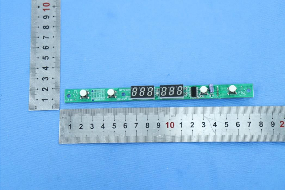
display board 3
