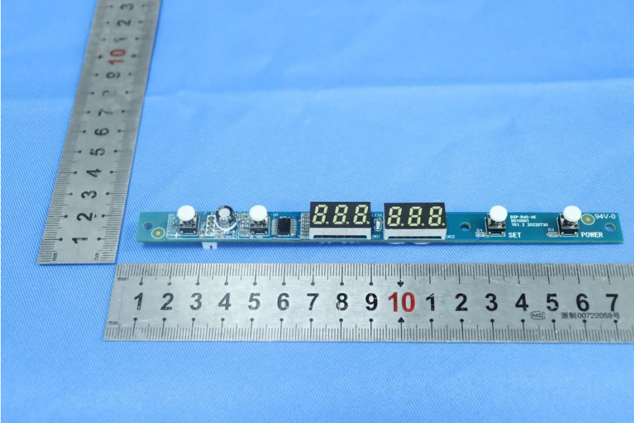
display board 4
