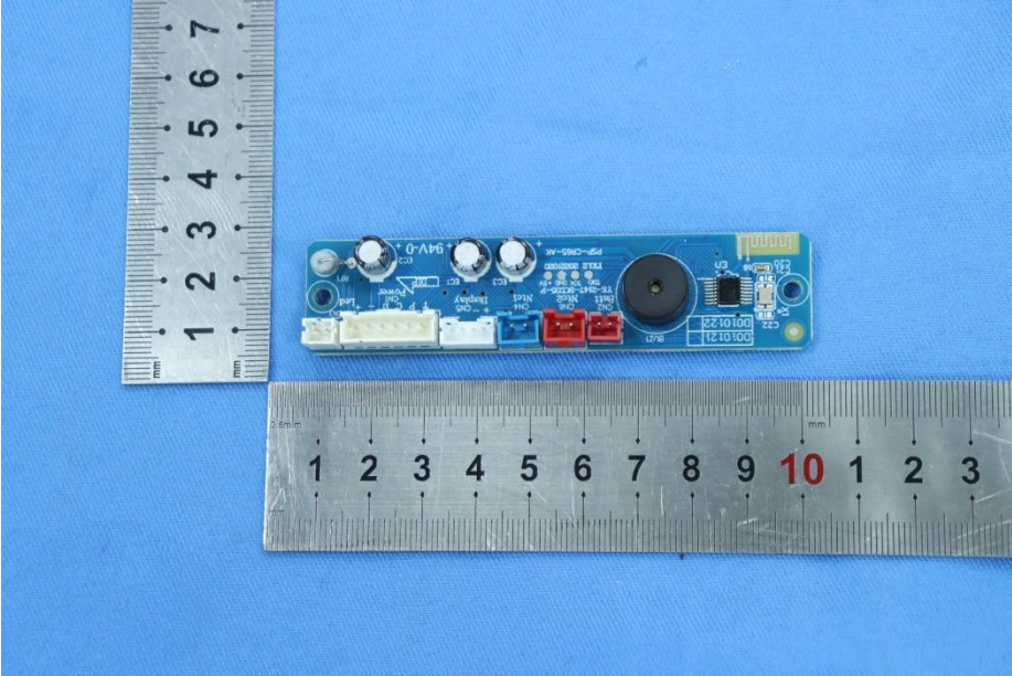
power board 2
