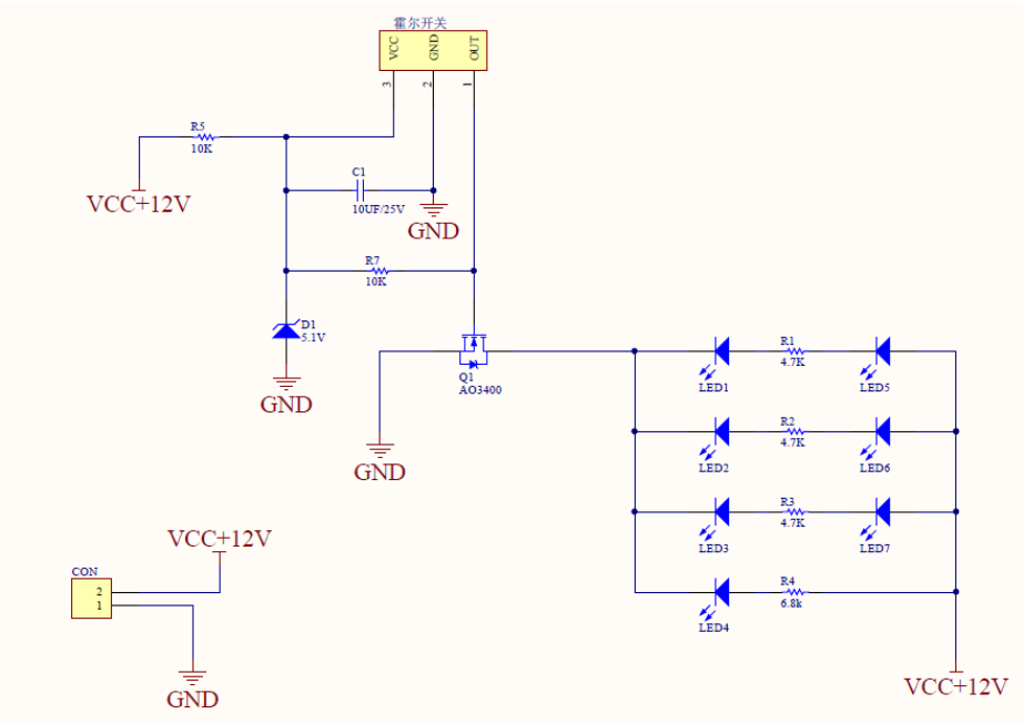
LED 1
