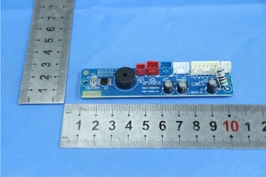
power board 4
