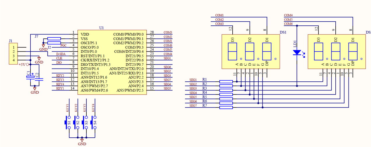
LED 1
